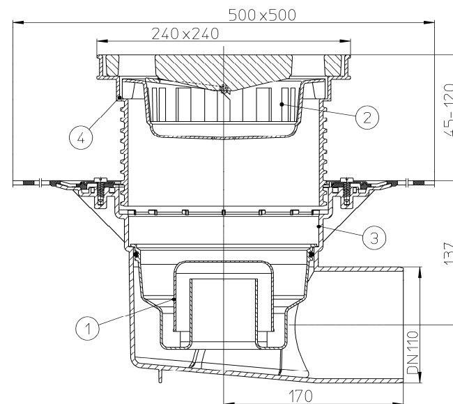
HL615HW
